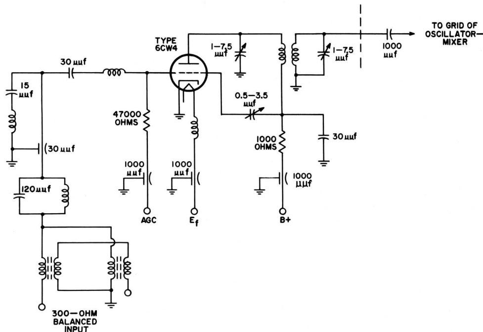
Fig.5 - Circuit diagram of the rf-amplifier section of an experimental turret tuner.
