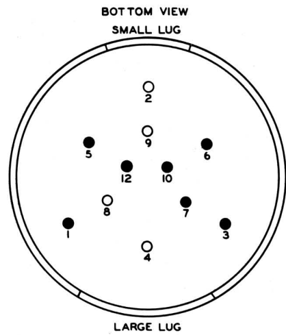
Fig.1 - Bottom view of pin arrangement for the 6CW4 and 2CW4.
