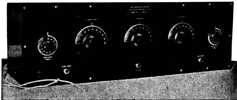
A HAZELTINE NEUTRODYNE RECEIVER
